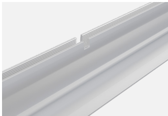
Main runners notched to positively position connectors on center every time
