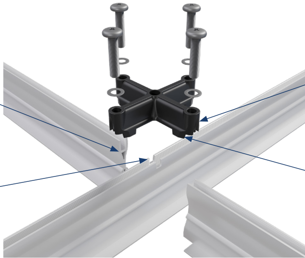
Field connector PN47690
