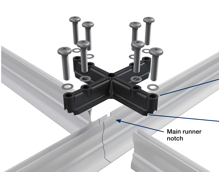
XL connector is designed for additional support at the ends of each main runner.
